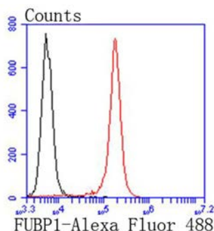
Fig. 3. Flow cytometric analysis of Jurakt cells with FUBP1 antibody at 1/50 dilution (red) compared with an unlabelled control (cells without incubation with primary antibody; black). Alexa Fluor 488-conjugated goat anti rabbit IgG was used as the secondary antibody.
